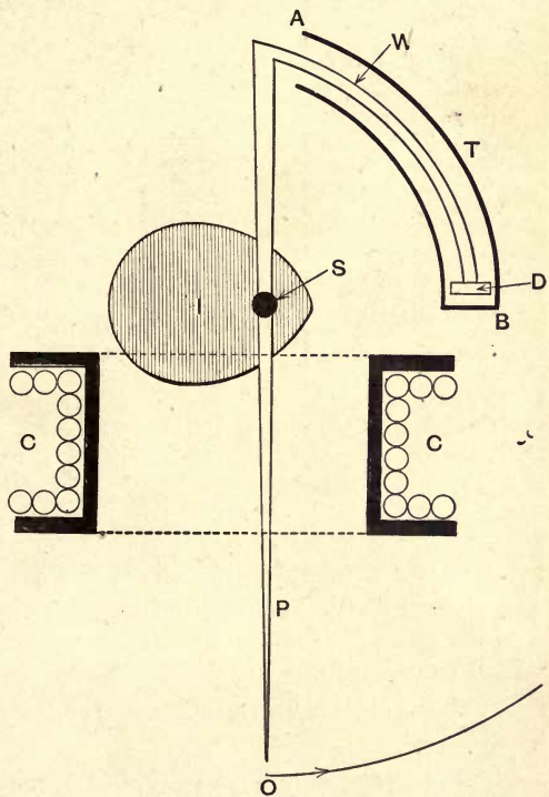
Fig. 22.—Working Principle of Moving-Needle Ammeter and Voltmeter (Siemens Bros. & Co.)
